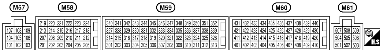
TCM (TRANSMISSION CONTROL MODULE)
