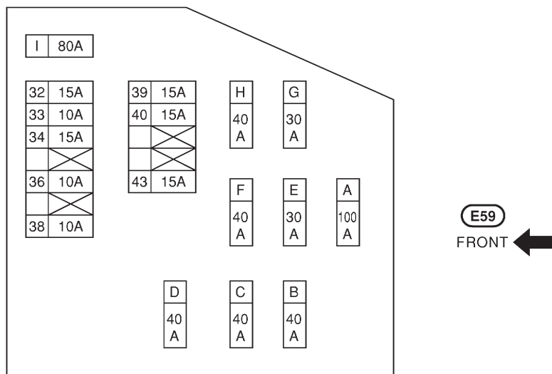
(QG engine models with daytime light system)
