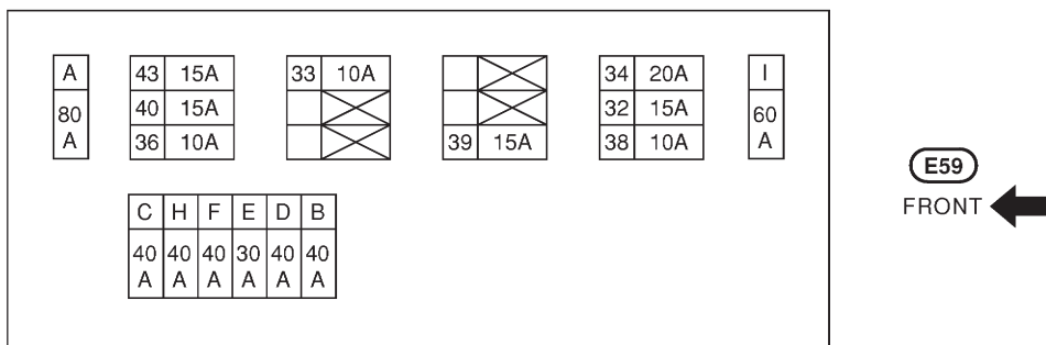
(QG engine models without daytime light system)
